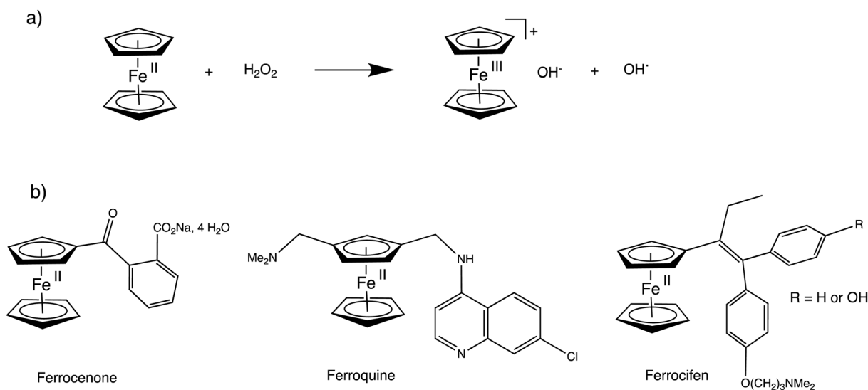
Fig. 18 (a) Fenton-type reaction of ferrocene partly responsible for ferrocene drug activity upon generating \text{OH}^* radicals at the vicinity of the sick cells; (b) main types of ferrocene-containing drugs.
