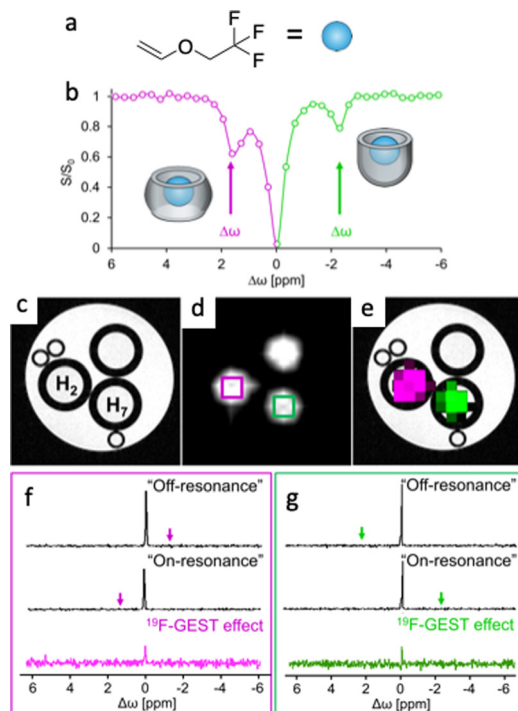
Fig. 9 Diamagnetic GEST: (a) the chemical structure of the fluorinated anesthetic fluorexene used as an inhalable ^{19}\text{F} -guest. (b) ^{19}\text{F} -NMR spectrum obtained from an aqueous solution containing a mixture of cucurbit[7]uril (H2) and dimeric octa acid (H7). The sample contained 5 mM fluorexene and 10 \mu\text{M} of each host. (c) ^1\text{H} -MRI, (d) ^{19}\text{F} -MRI, and (e) ^{19}\text{F} -GEST map of a three-tube phantom containing 5 mM fluorexene and 5 \mu\text{M} of either cucurbit[7]uril (H2) or octa acid (H7). A tube with 5 mM fluorexene only was used as a control. (f and g) Localized ^{19}\text{F} -GEST spectroscopy data of two voxels acquired from the tubes containing (f) H2:fluorexene (magenta) or (g) H7:fluorexene (green). The ^{19}\text{F} -GEST spectra represent the subtraction of the ^{19}\text{F} -NMR spectra obtained when the saturation pulse was applied "on-resonance" from the ^{19}\text{F} -NMR spectra obtained when the saturation pulse was applied "off-resonance." Data were acquired with a 9.4 T MRI scanner with B_1 = 2.5 \mu\text{T}/2 \text{ s} . For fluorexene@H2, "on-resonance" was \Delta\omega = +1.6 \text{ ppm} and "off-resonance" was \Delta\omega = -1.6 \text{ ppm} . For fluorexene@H7, "on-resonance" was \Delta\omega = -2.2 \text{ ppm} and "off-resonance" was \Delta\omega = +2.2 \text{ ppm} . Modified with permission from ref. 83.
