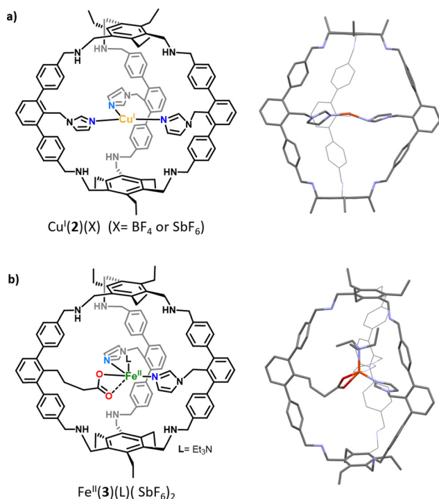
Fig. 2 Schematic representations and XRD structures of (a) the confined copper complex \text{Cu}^{\text{I}}(\mathbf{2}) and (b) heteroleptic caged iron complex \text{Fe}^{\text{II}}(\mathbf{3}) .
