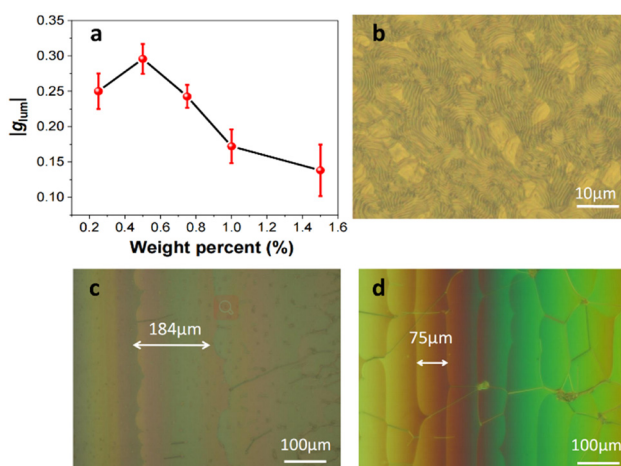
Fig. 2 (a) The tendency of CPL g_{\text{lum}} values with different mixing weight ratios of R -1-C, \lambda_{\text{ex}} = 360 nm, all error bars show the mean \pm standard deviation, n = 5 independent experiments. (b) POM image of R -1-C/E7, [ R -1-C] = 0.5 wt%. POM images of N*-LC including 0.5 wt% (c) R -1-O and (d) R -1-C in wedge-shaped cells at room temperature.
