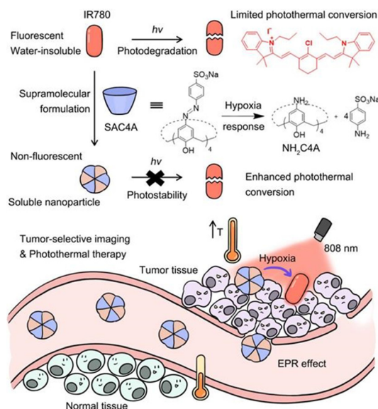
Fig. 19 Schematic illustration of supramolecular PTA formed by host-guest complexation between SAC4A and IR780 and the effect of photo-thermal therapy on cancer cells. Reproduced with permission from ref. 113. Copyright 2022 Ivy-Spring.
