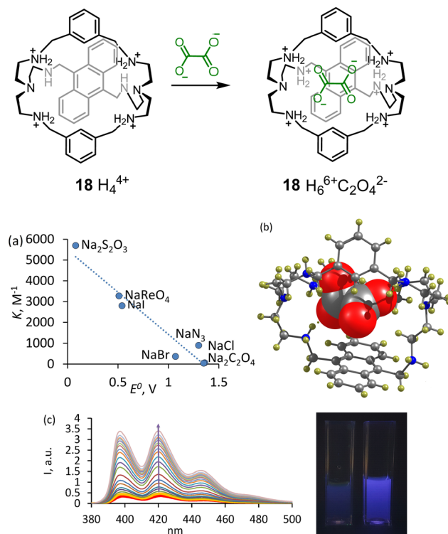
Fig. 7 Complexation of 18 with oxalate. (a) Correlation between Stern–Volmer quenching and reduction potentials of the anions. (b) Molecular structure of the oxalate complex according to the single X-ray crystal analysis. Reproduced from ref. 41 with permission from the Royal Society of Chemistry. (c) Fluorescence changes observed upon gradual addition of oxalate to 18 . The cuvettes show the fluorescence of 18 under UV-lamp without oxalate and with 10 equiv. of oxalate.
