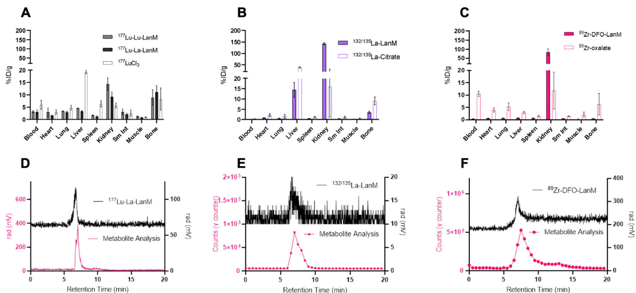
Fig. 4 (A) Two-hour post-injection biodistribution analysis of [ 177 Lu]-LanM using nat Lu ( 38 \mu\text{Ci nmol}^{-1} , 68\text{--}77 \mu\text{Ci} administered per mouse, n = 3 ) or nat La ( 35 \mu\text{Ci nmol}^{-1} , 56\text{--}75 \mu\text{Ci} administered per mouse, n = 4 ) as carrier in direct comparison with the distribution of 177 LuCl 3 as the free ion surrogate ( n = 3 ). (B) Two-hour post-injection biodistribution analysis of [ 132/135 La]-LanM ( 4 \mu\text{Ci nmol}^{-1} , 10\text{--}14 \mu\text{Ci} administered per mouse, n = 3 ) with nat La as carrier in direct comparison with the distribution of 132/135 La-citrate as the free ion surrogate ( n = 3 ). (C) Two-hour post-injection biodistribution analysis of [ 89 Zr]-DFO-LanM ( 40 \mu\text{Ci nmol}^{-1} , 25\text{--}40 \mu\text{Ci} administered per mouse, n = 5 ) in direct comparison with the distribution of 89 Zr-oxalate as the free ion surrogate ( n = 3 ). (D) SEC-HPLC and urine metabolite analysis of [ 177 Lu]-LanM using nat La as non-radioactive carrier (E) SEC-HPLC and urine metabolite analysis of [ 132/135 La]-LanM. (F) SEC-HPLC and urine metabolite analysis of [ 89 Zr]-DFO-LanM.
