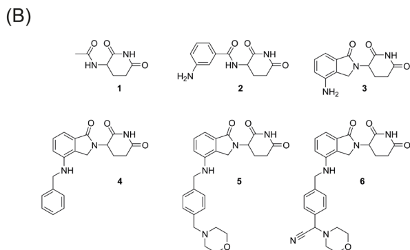
Fig. 2 (A) The crystal structure of CRBN in complex with CC-220 (PDB: 5V3O) 16 reveals a possible exit vector for linker attachment. (B) Strategy towards three-branched CRBN recruiters: stepwise increase of the ligand size and incorporation of an exit vector by multicomponent reactions.
