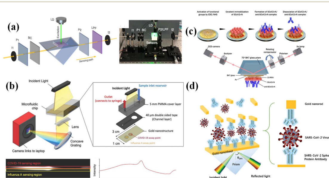
Fig. 6 (a) Schematic and experimental setup of the dual-functional PPT-enhanced LSPR biosensing system. Reproduced with permission from ref. 127. (b) Scheme of the SPR spectral imaging platform integrated with a microfluidic chip. A typical spectral image is shown, and it was obtained from the CCD. Reproduced with permission from ref. 128. (c) Schematic representation of the gold-coated sensor disk (Au-disk) surface modified with antigen SCoV2-rN, which was applied as an interactive surface. Reproduced with permission from ref. 129. (d) The SPR biosensor was designed using a sandwich structure. Reproduced with permission from ref. 130.
