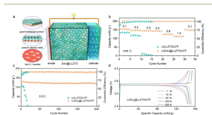
Fig. 5 (a) Schematic construction of the Li/ \text{ZnI}_2 @LLZTO/LFP full cell. (b) Rate performance of Li/SSE/LFP full cells with \text{ZnI}_2 @LLZTO or LLZTO in 2.5–4.1 V. (c) The cycling performance of full cells at 0.5C. (d) Charge–discharge profiles of the Li/ \text{ZnI}_2 @LLZTO/LFP full cell at 0.5C.
