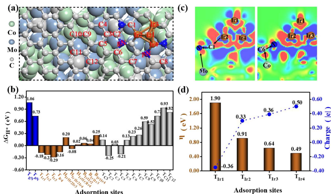
Fig. 5 (a) The theoretical model used in DFT calculations and the obtained adsorption sites on the model surface; (b) the calculated free energies of H + adsorption ( \Delta G_{H^*} ) for these adsorption sites; (c) the charge density difference ( \Delta\rho ) of the composite Co 6 Mo 6 C-Ir NF system, in which the red and blue colors represent gaining and losing electrons, respectively, and the relevant electron transfer processes are displayed; (d) the overpotential \eta values of the OER on the surface of the composite Co 6 Mo 6 C-Ir NF system and the Bader charge of the corresponding active sites.
