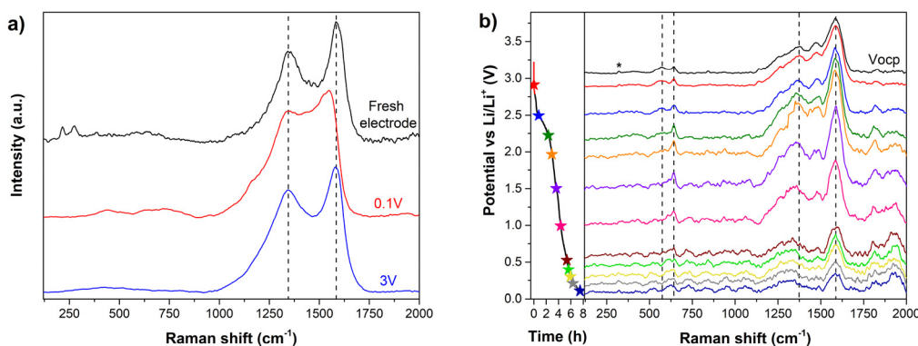
Fig. 5 (a) Ex situ Raman measurements of two fully activated electrodes stopped at 0.1 V (lithiated) and 3 V (delithiated) and a fresh non-cycled electrode. The three spectra have been normalized to facilitate comparison. (b) Operando Raman spectra of the first galvanostatic lithiation measured at the voltages indicated in the plot profile on the left. The asterisk indicates the peak from the CaF 2 window of the Raman cell used for the operando Raman measurements.
