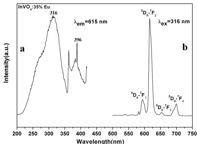
Fig. 6 Photoluminescence spectra and illustration of \text{InVO}_4\text{:}30\% \text{Eu}^{3+} .
