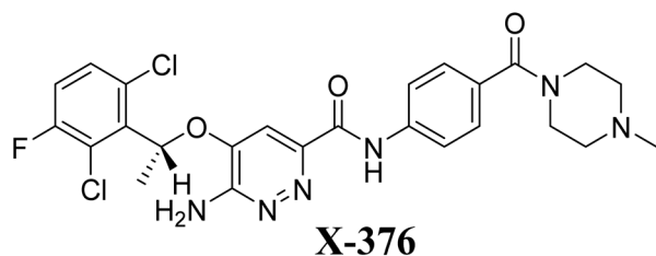
Fig. 1 Chemical structure of X-376 .
