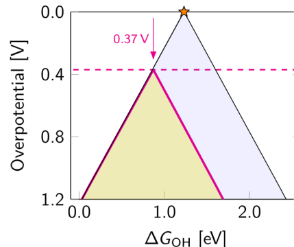
Fig. 7 Projection of the three-dimensional overpotential volcano for ORR along \Delta G_{\text{OH}} axis. The dashed magenta line indicates achievable overpotentials within the OOH–OH scaling relation with the lowest value of 0.37 V further from the ideal catalyst.
