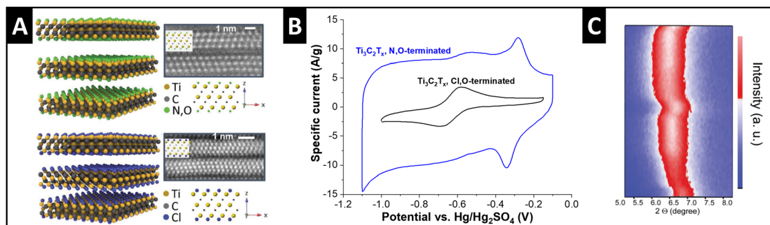
Fig. 5 Solvent coinercation by tuning nanoconfinement chemistry in MXenes. (A) Structural models and transmission electron micrographs (high-angle annular dark-field) of N,O- and Cl-terminated \text{Ti}_3\text{C}_2\text{T}_x MXenes, (B) their cyclic voltammograms in 3 M \text{H}_2\text{SO}_4 electrolyte at 20 \text{mV s}^{-1} , and (C) in situ XRD heatmap for two full galvanostatic cycles of the N,O-terminated electrode, replotted or adapted with permission from ref. 51, Copyright 2023 John Wiley & Sons.
