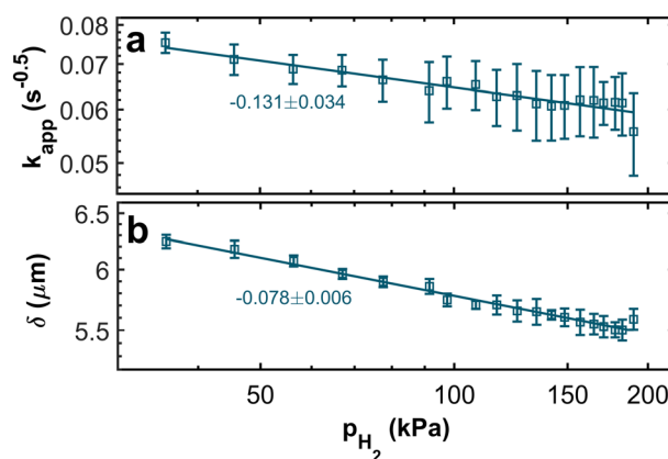
Fig. 8 Double-logarithmic plots of (a) the apparent rate coefficient k_{app} and (b) the Nernst diffusion layer thickness \delta in relation to the hydrogen partial pressure.
