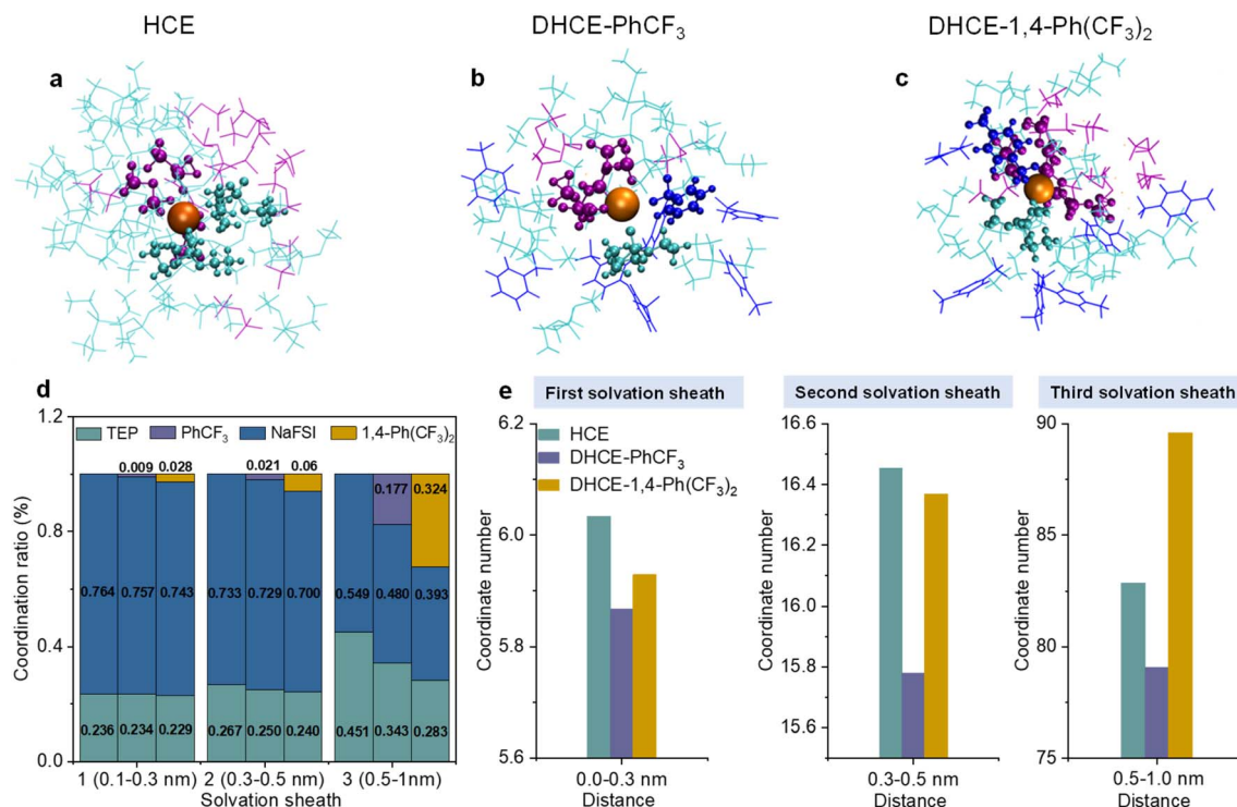
Fig. 1 Representative Na + solvation structures of (a) HCE, (b) DHCE-PhCF 3 , and (c) DHCE-1,4-Ph(CF 3 ) 2 extracted from MD simulations. The TEP, FSI − , Na + , and diluents (PhCF 3 and 1,4-Ph(CF 3 ) 2 ) are shown in cyan, purple, orange, and blue, respectively. The TEP, FSI − , and diluents (PhCF 3 and 1,4-Ph(CF 3 ) 2 ) in the Na + primary solvation sheath are depicted using a ball-and-stick model, while the wireframes stand for the second and third solvation sheaths. (d) The coordination ratios of different electrolytes at different solvation sheaths extracted from MD simulations. The bars in each solvation sheath (0–0.3 nm, 0.3–0.5 nm, 0.5–1 nm) represent HCE, DHCE-PhCF 3 , and DHCE-1,4-Ph(CF 3 ) 2 electrolytes from left to right, respectively. (e) The coordination numbers of Na + in different electrolytes at different solvation sheaths extracted from MD simulations.
