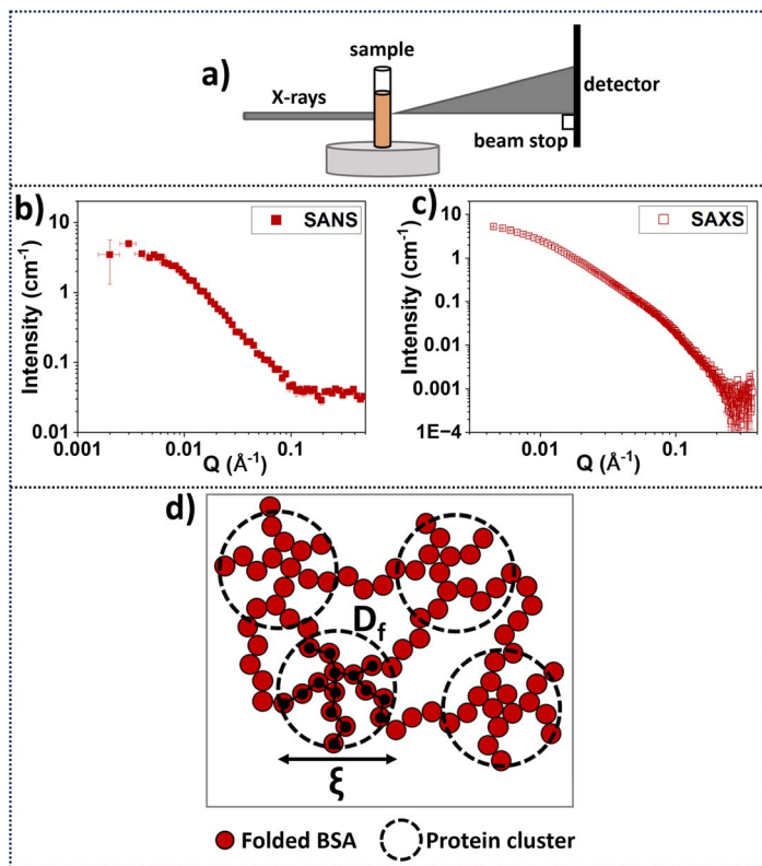
Fig. 3 (a) Schematic of SAXS data acquisition geometry. The accessible q -range investigated in the Hughes et al. study 70 was 0.0045\text{--}0.37\ \text{\AA}^{-1} and 0.002\text{--}0.5\ \text{\AA}^{-1} for SAXS and SANS, respectively. Samples were directly gelled inside sample holders. 70 (b) SANS data 70 from the Sans2d instrument at the ISIS neutron and Muon Source, UK, for folded BSA hydrogels (concentration: 7.4% BSA, 20 mM NaPS, 100 \mu\text{M} Ru(BiPy) 3 in 35% D 2 O/65% H 2 O and (c) SAXS data 70 from Nano-inXider instrument at the ISIS neutron and Muon Source for folded BSA hydrogels (concentration: 7.4% BSA, 20 mM NaPS, 100 \mu\text{M} Ru(BiPy) 3 in 100% H 2 O). 70 (d) Schematic of the predicted network structure using SANS and SAXS using model fitting of the data 70 suggesting that the network consists of connected clusters made by folded protein. Correlation length \xi is indicative of the cluster size, and the fractal dimension D_f can be thought of as the density of the cluster.
