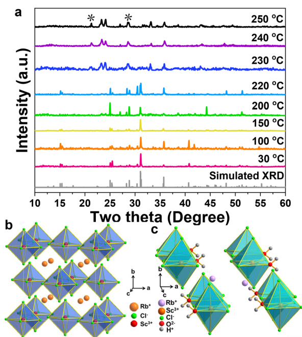
Fig. 4 (a) XRD patterns of \text{Rb}_2\text{ScCl}_5 \cdot \text{H}_2\text{O}:\text{Sb}^{3+} treated at different temperatures. The asterisks denote the impurity of \text{RbScCl}_4 . Structure projection of (b) \text{Rb}_3\text{ScCl}_6 and (c) \text{Rb}_2\text{ScCl}_5 \cdot \text{H}_2\text{O} crystals plotted using the software Diamond 3.1.
