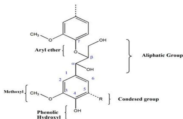
Figure 2. The main functional group in lignin's structure. Reproduced from Gonçalves et al., Polymers , 2021, 13, 4196, licensed under CC BY 4.0
