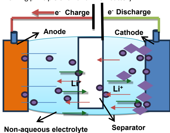
Figure 1. Working principle of a lithium-ion cell. Adapted from Ghiji et al., Energies 2020, 13, 5117, licensed under CC BY 4.0
