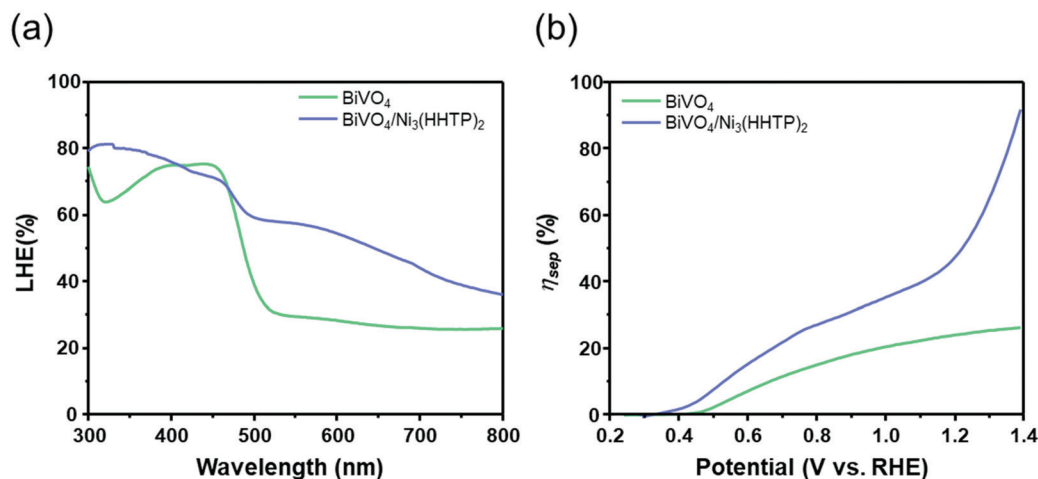
Fig. 5 (a) Light harvesting efficiency (LHE) (%) and (b) charge separation efficiency ( \eta_{\text{sep}} ) of \text{BiVO}_4 and \text{BiVO}_4/\text{Ni}_3(\text{HHPT})_2 .
