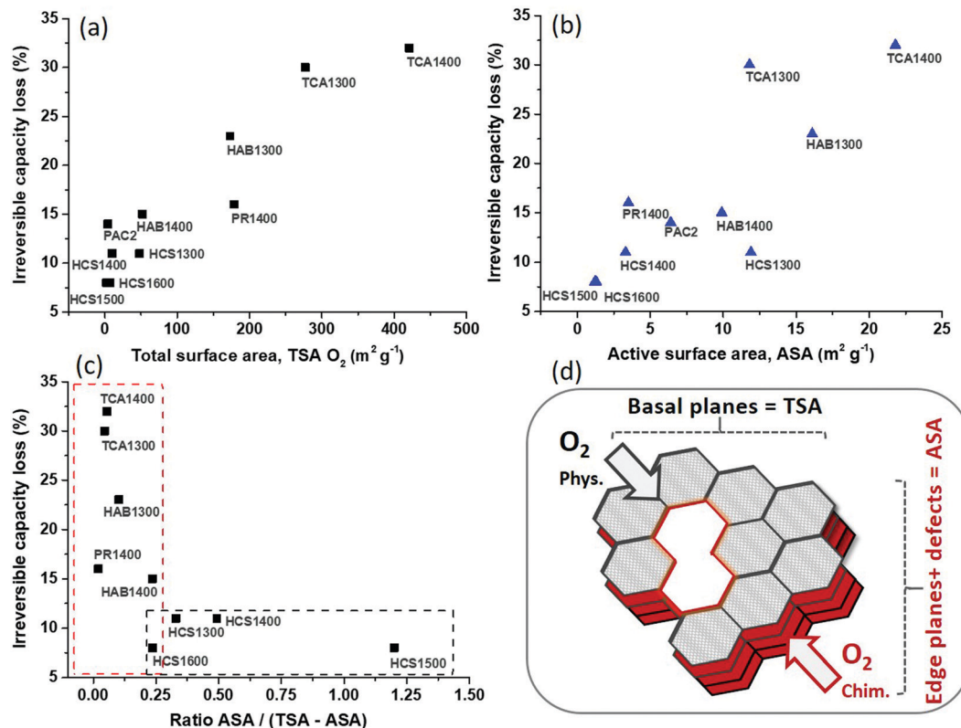
Fig. 3 Relationship between the 1st irreversible capacity loss and (a) total surface area ( TSA_{O_2} ), (b) active surface area ( ASA ), (c) ratio ASA/(TSA_{O_2}-ASA) . (d) Representation of hard carbon structure containing the active surface (edge planes and defects) and the basal planes surface ( TSA-ASA ).
