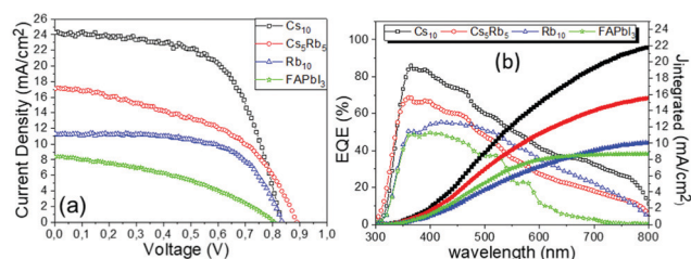
Fig. 3 (a) Current density–voltage curves of the champion C-PSCs, incorporating the MA-free perovskites under study, the champion illumination of 100\text{ mW cm}^{-2} simulated sun irradiation (1.5 AM) and (b) EQE of the corresponding solar cells.
