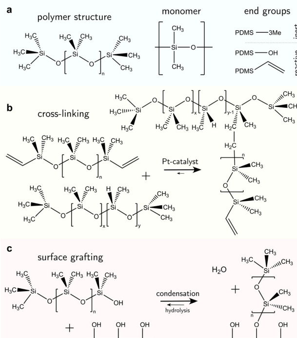
Fig. 2 Chemical structure of polydimethylsiloxane. (a) PDMS can be oligomeric ( n < 100 ) with low viscosity (1–5 mPa s) or assemble into long chains with high viscosities (up to \eta = 10 \text{ kPa s} ). The silicon–oxygen backbone provides chain flexibility while the methyl side chains yield water repellency. The end groups can be inert (trimethylsilyl) or reactive (hydroxyl, vinyl). (b) Hydrosilylation reaction between linear vinyl-terminated PDMS chains (top) and cross-linking agents with methylhydrosiloxane monomers create branches and networked elastomeric polymers. Here, the cross-linking agent is a polymer chain with x dimethylsiloxane and y methylhydrosiloxane monomers that are randomly arranged. The network branches are randomly distributed on the cross-linker chain and terminal on the PDMS base chain. (c) Hydroxyl-terminated PDMS chains can be grafted on surface hydroxyl groups that naturally occur on metals/metal-oxide, or can be functionalized with hydrogen plasma.
