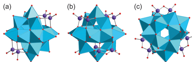
Fig. 6 Polyhedral representations of the "fully-reduced" SiPOVs [V_{16}Si_4O_{46}]^{12-} (a), \alpha-[H_4V_{14}O_{44}(SiO)_8]^{12-} (b), and [V_{15}Si_6O_{42}(OH)_6]^{6-} (c). Encapsulated H_2O (a and b), Cl^- (c), and hydrogen atoms are not shown. Colour code: Si, violet; O, red spheres; V^{IV}O_x , sky-blue polyhedra.
