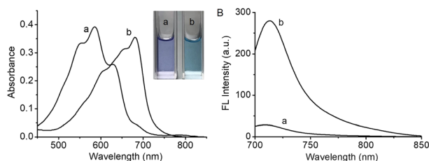
Fig. 1 The absorption (A) and fluorescence (B) spectra of HCH-AcAH (10 \mu\text{M} ) before (a) and after (b) reacting with CES (200 U \text{L}^{-1} ). \lambda_{\text{ex}} = 680 nm.
