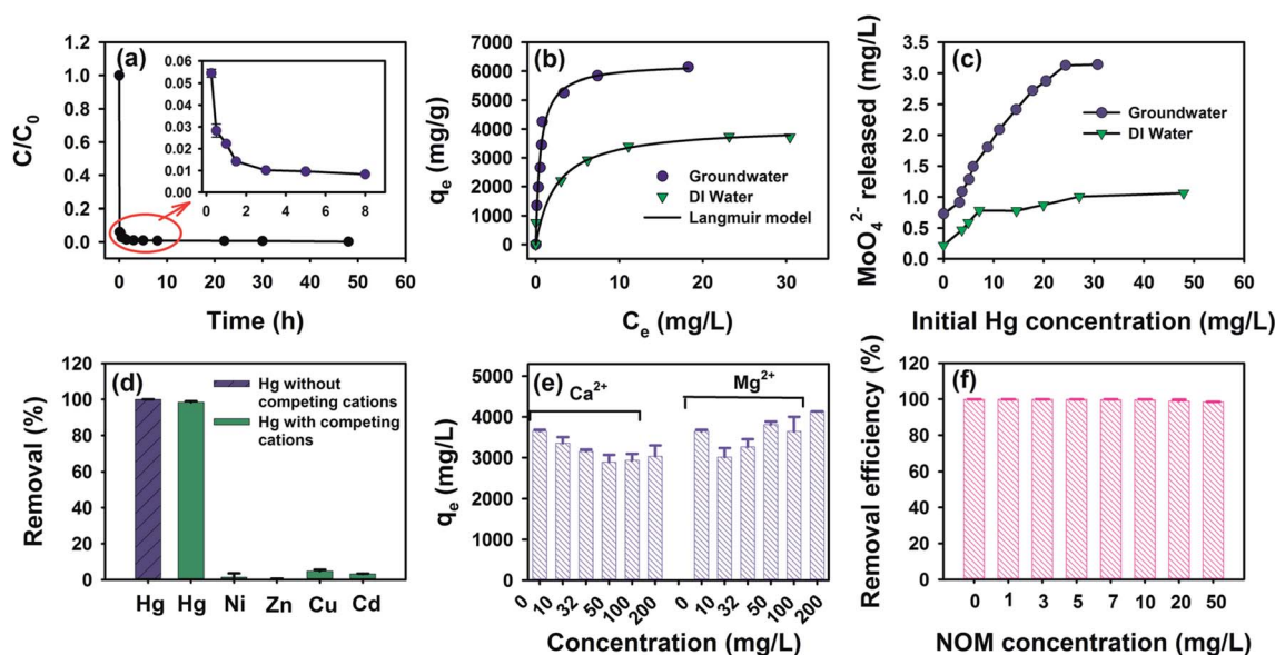
Fig. 2 Hg(II) removal by MoS 2 nanosheets. (a) Kinetics of Hg(II) uptake by MoS 2 nanosheets, C_{\text{Hg}} = 5 \text{ mg L}^{-1} and C_{\text{MoS}_2} = 4 \text{ mg L}^{-1} ; (b) isotherm of Hg(II) uptake by MoS 2 fitted with Langmuir model, C_{\text{Hg}} = 0\text{--}42 \text{ mg L}^{-1} ; (c) the concentration of MoO 4 2- in the solution after reaction between MoS 2 and Hg ions; (d) removal efficiency of various heavy metals by MoS 2 nanosheets in a mixture containing all cations at equal concentrations of 1 mg L -1 ; (e) effects of Ca(II) and Mg(II) on Hg removal by MoS 2 nanosheets; (f) effects of NOM on Hg removal by MoS 2 , C_{\text{Hg}} = 20 \text{ mg L}^{-1} and C_{\text{MoS}_2} = 15 \text{ mg L}^{-1} .
