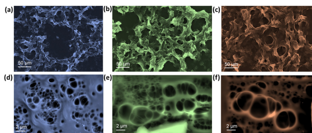
Fig. 5 SEM microstructure images of the HPC-PAA hydrogel at (a)–(d) 4 ^{\circ}\text{C} , (b)–(e) 22 ^{\circ}\text{C} , and (c)–(f) 45 ^{\circ}\text{C} for different magnifications, respectively.
