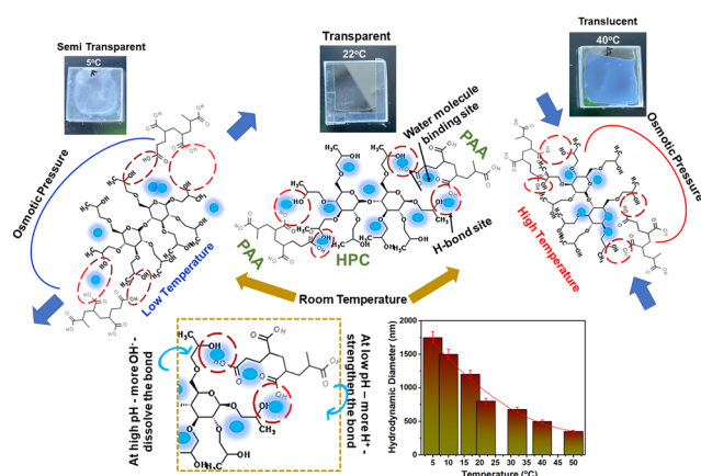
Fig. 7 Schematic representation of the possible temperature-pH-transparency tuning mechanism of the HPC–PAA hydrogel for optimal climate-adaptable energy saving smart windows along with temperature-dependent DLS measurements.
