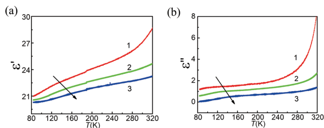
Fig. 4 Temperature dependence of the \text{SnP}_2\text{S}_6 crystal dielectric permittivity of the real (a) and imaginary (b) parts at frequencies 1(1 kHz), 2(10 kHz), and 3(40 kHz).
