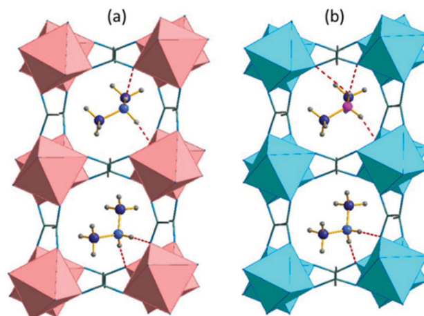
Fig. 3 The crystal structure of the low-temperature phase (a) [(CH 3 ) 2 NH 2 ]Mn(HCOO) 3 , 100 K, the monoclinic Cc model taken from ref. 43; and (b) [(CH 3 ) 2 NH 2 ]Zn(DCOO) 3 triclinic, P1 . The inequivalent nitrogen positions are marked by blue and fuchsia.
