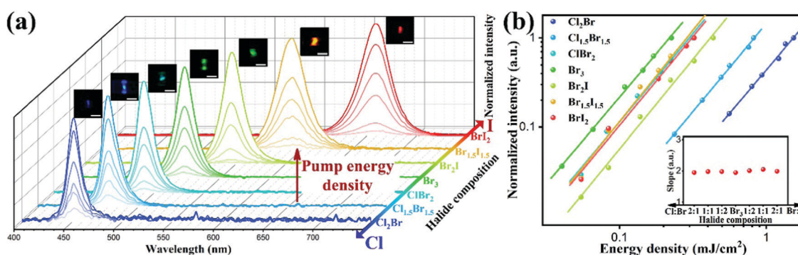
Fig. 3 (a) Two-photon excited luminescence of the ZJU-28 CsPbX 3 crystals under fs pulsed laser excitation at 780 nm (for X 3 = Cl 2 Br, Cl 1.5 Br 1.5 , ClBr 2 and Br 3 ) or 980 nm (for X 3 = Br 2 I, Br 1.5 I 1.5 and BrI 2 ). Insets: The microscopy images of ZJU-28 CsPbX 3 crystals upon infrared fs pulsed laser excitation. Scale bar, 50 μm. (b) Pump energy density-dependent 2PE emission intensity of the ZJU-28 CsPbX 3 crystals. The inset displays the slopes of the logarithm of the emission intensity and the logarithm of the pump energy. Test environment: temperature of 25 °C, humidity of 55%.
