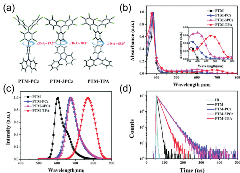
Fig. 6 (a) Molecular geometries of substituted PTM radicals (DFT (UB3LYP/6-31G(d)). (b) UV-Vis absorption, (c) PL and (d) fluorescence lifetime of the radicals in cyclohexane solution (concentration: 10^{-5} \text{ M} , excitation wavelength: 380 nm). Reproduced with permission from ref. 90 Copyright the Owner Societies 2018.
