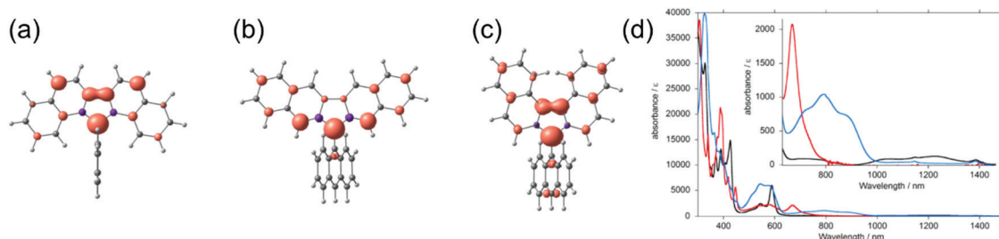
Fig. 9 Spin density maps of (a) 9 , (b) 10 and (c) 11 calculated with UBLYP/6-31G**//UB3LYP/6-31G** method. Red and purple surfaces represent \alpha and \beta spin densities drawn at 0.004 \text{ e a.u.}^{-3} level, respectively. (d) UV-Vis-NIR spectra ( 1.0 \times 10^{-4} \text{ M} in \text{CH}_2\text{Cl}_2 , room temperature) of 9 (black line), 10 (red line), and 11 (blue line). Inset shows a magnified view in the NIR region. Reprinted (adapted) with permission from ref. 130 Copyright 2014 American Chemical Society.
