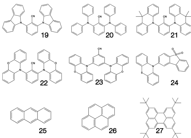
Fig. 3 Charge transfer (19–24) and polycyclic aromatic (25–27) type structures considered in this work.
