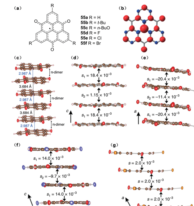
Fig. 20 (a) 4,8,12-Trioxotriangulene radical structure, (b) DFT calculated (the UBLYP/6-31G** level) electronic spin density distribution, and their X-ray crystallographic structure with 1D \pi -stacked radical columns of (c) 55a , (d) 55b , (e) 55c , (f) 55d and (g) 55f and intermolecular overlap integrals. Adapted with permission from ref. 96, Springer Nature.
