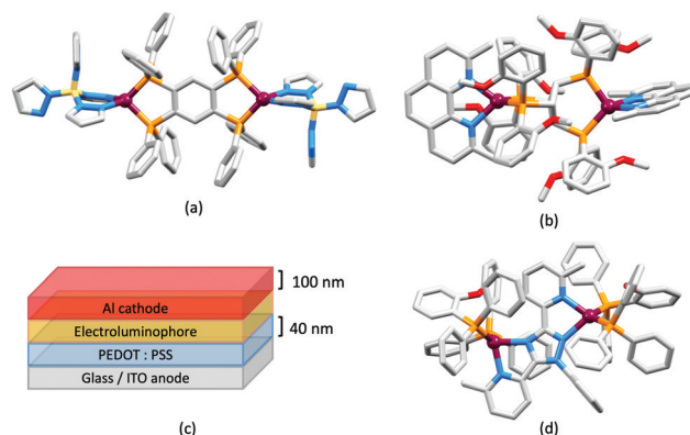
Fig. 22 Structures of (a) [Cu 2 (pz 4 B) 2 (μ-tpbz)] (CSD refcode KURCAD), and (b) the cationic complex in [Cu 2 (2,9-Me 2 phen) 2 (μ-MeOdpccb)][PF 6 ] 2 (refcode VOZQAE). (c) Architecture of a LEC containing [Cu 2 (2,9-Me 2 phen) 2 (μ-MeOdpccb)][PF 6 ] 2 in the active layer; the LEC was driven under a bias of 4 or 5 V. (d) Structure of the dinuclear cation in [Cu 2 (POP) 2 (μ- 37 )][BF 4 ] 2 (refcode MAMXUW). H atoms are omitted from the figures for clarity.
