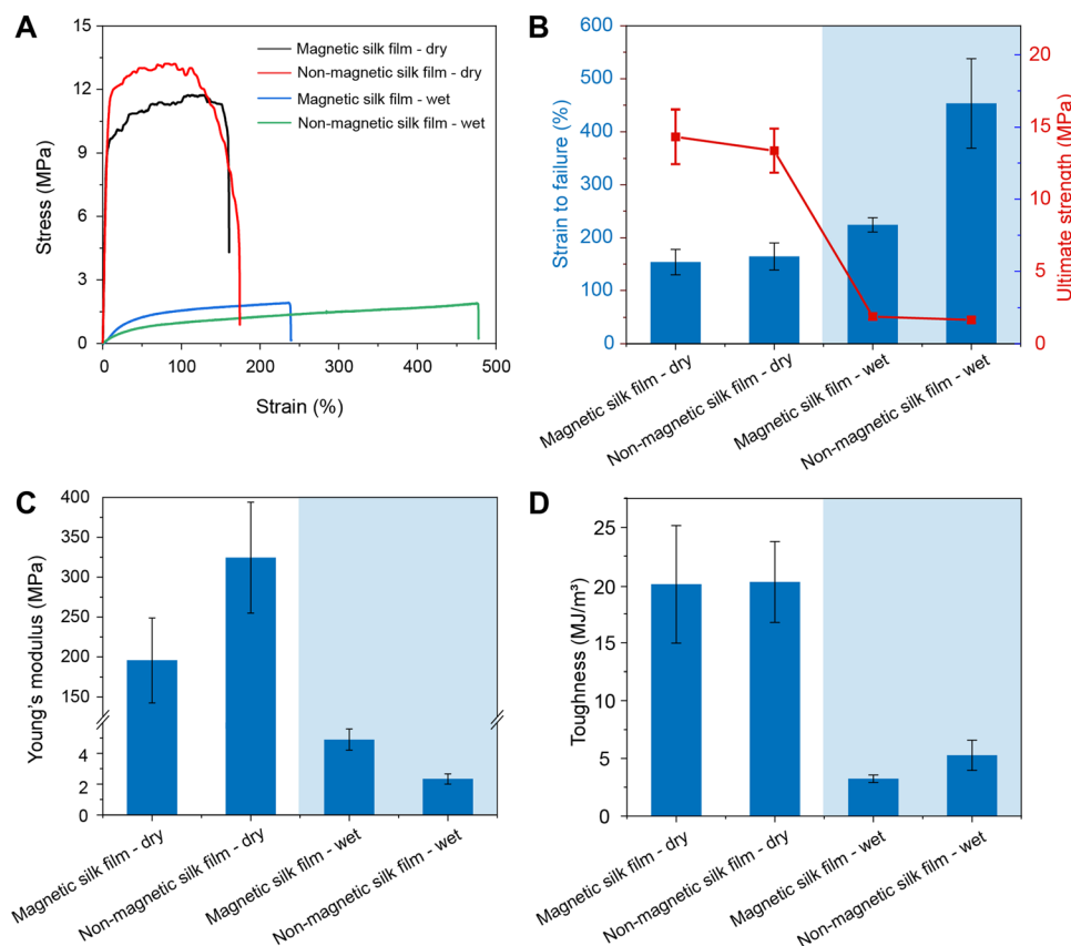
Fig. 4 (A) Representative stress–strain curves of the magnetic and non-magnetic silk films under dry and wet conditions. The summary of strain at failure, ultimate strength (B), Young's modulus (C), and toughness (D) of the magnetic and non-magnetic silk films under dry and wet conditions.
