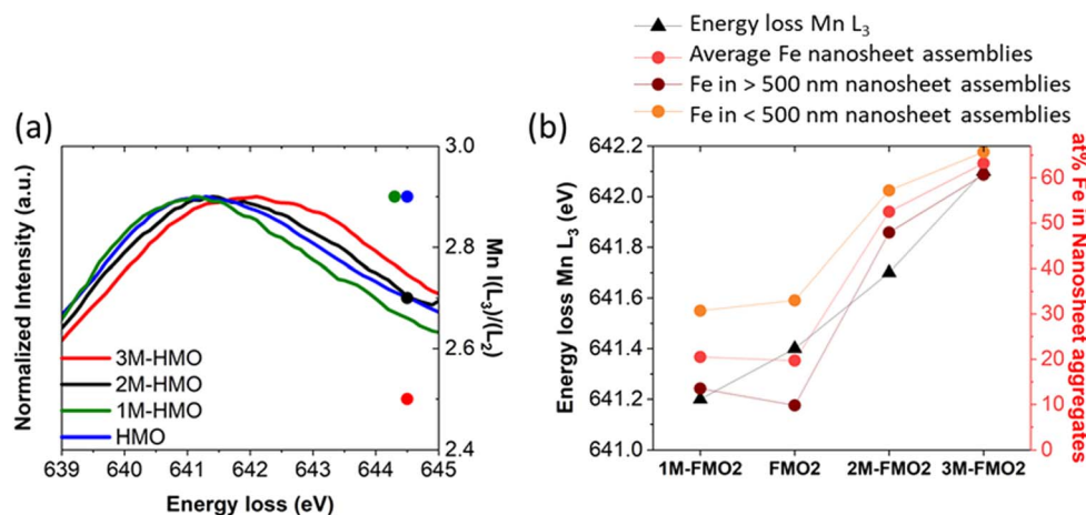
Fig. 8 (a) Left-Y Axis: EELS Mn L_3 peaks of HMO, 1M-HMO, 2M-HMO and 3M-HMO. Right-Y axis: corresponding \text{Mn } I(L_3)/I(L_2) values. (b) Trends of oxidation state of xM-HMO (Left-Y axis) and Fe introduced by galvanic exchange reaction (right-Y axis) for xM-FMO2.
