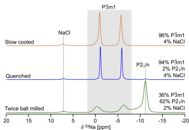
Fig. 2 23 Na ss-NMR spectra for twice ball milled (bottom), quenched (middle), and slow cooled (top) \text{Na}_2\text{ZrCl}_6 samples. Resonances assigned to the P\bar{3}m1 polymorph are within the grey box, while the prismatic Na site of the P2_1/n structure is on the dotted line to its right. For each sample, the molar% of Na in each phase is shown on the right hand side of the spectrum. Spectra were obtained at a 10 kHz spinning speed, resulting in a sample temperature of 52 °C.
