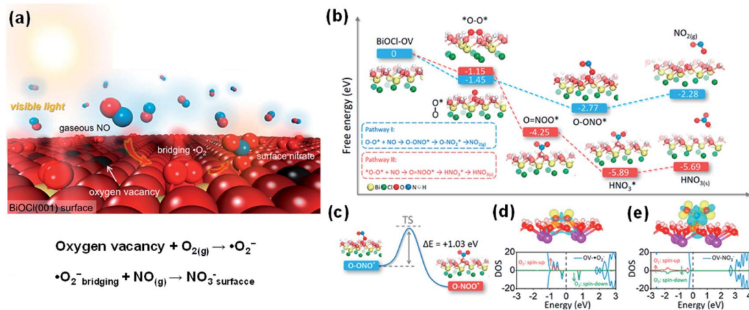
Fig. 16 (a) Schematic illustration of photocatalytic NO removal by BiOCl-OV. (b) Free energy change against the reaction coordinate for the oxidation of NO by O _2^{\cdot-} on the BiOCl (001) surface in different geometries. (c) Geometric transition from peroxynitrite to nitrate. TS represents the transition state. Charge density difference and O _2 partial DOS of the BiOCl (001) surface adsorbed with (d) O _2 and (e) nitrate. The yellow and blue isosurfaces with an iso-value of 0.005 au represent charge accumulation and depletion in space. The vertical dashed line in the DOS shows the VBM. Adapted with permission from ref. 247 Copyright (2018) American Chemical Society.
