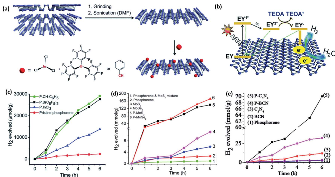
Fig. 8 (a) Schematic representation of liquid exfoliation of BP into phosphorene nanosheets and their functionalization with InCl 3 , B(C 6 F 5 ) 3 and benzyl group. (b) Plausible mechanism of eosin Y sensitised photocatalytic HER in the presence of TEOA as a sacrificial agent. (c) Hydrogen evolved versus time plots of pristine and functionalized phosphorenes. (d) Hydrogen evolved versus time plots of covalently cross-linked phosphorene–MoS 2 and phosphorene–MoSe 2 composites. (e) Hydrogen evolved versus time plots of metal-free covalently cross-linked phosphorene–C 3 N 4 and phosphorene–BCN composites. Panels (a–c) reproduced with permission from ref. 11, © 2019. The Royal Society of Chemistry. Panel (d) reproduced with permission from ref. 48, © 2019 American Chemical Society. Panel (e) reproduced with permission from ref. 54, © Author(s) 2020.
