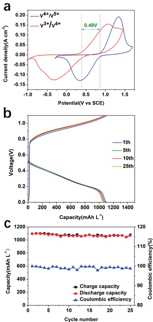
Fig. 4 (a) CV in 0.1\ M\ V^{3+}/V^{4+} and V^{4+}/V^{5+} , with a three-electrode electrochemical cell using, in 3.0\ M\ H_2SO_4 , carbon felt, an SCE and a Pt coil as the working, reference, and counter electrodes, respectively. (b) Charge/discharge experiments for a redox flow cell using 1.0\ M\ V^{4+} , 3.0\ M\ H_2SO_4 electrolyte, and a current density of 1.0\ mA\ cm^{-2} from 0\ V to 1.1\ V . (c) Charge–discharge capacity and coulombic efficiency of the RFB.
