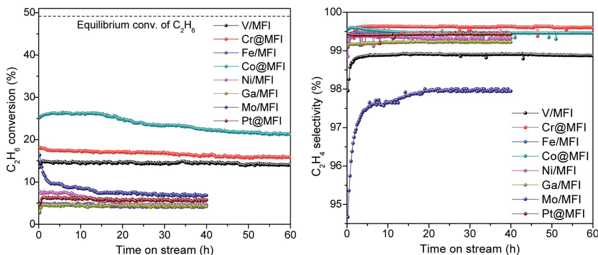
Fig. 1 EDH activities of different metal catalysts. Reaction conditions: 100 mg catalyst, pretreatment by 10% H 2 /N 2 for 30 min, 20% C 2 H 6 /N 2 , 10 mL min -1 , 1 bar, 650 °C.
