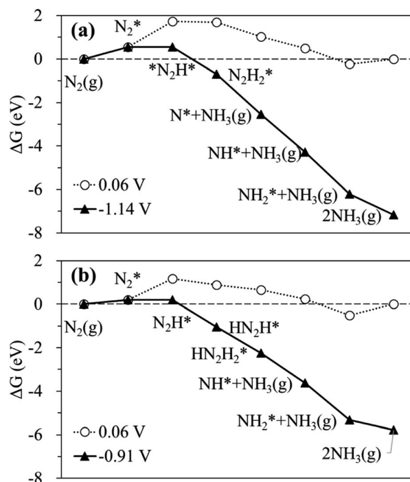
Fig. 3 Calculated free energy profiles at equilibrium (O) and limiting (▲) potentials for the N_2RR on (a) the Ru SAC and (b) the homo- Ru_2 DAC via the most favourable pathway.
