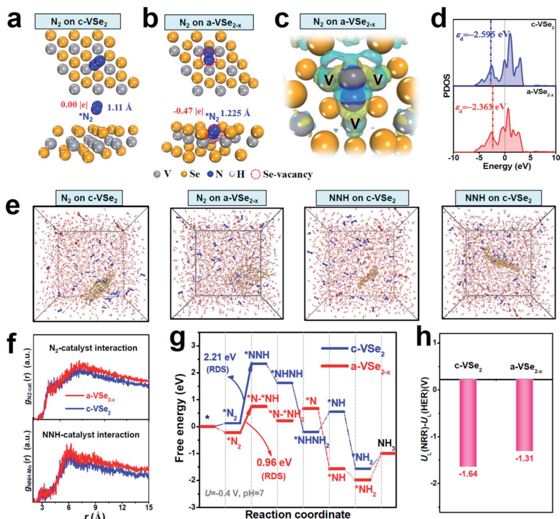
Fig. 4 (a and b) Optimized structures of *N 2 on c-VSe 2 and a-VSe 2-x . (c) Electron deformation density of *N 2 on a-VSe 2-x . Yellow and cyan isosurfaces represent electron accumulation and electron depletion, respectively. (d) PDOS of V-3d in c-VSe 2 and a-VSe 2-x for determining the d-band center ( \epsilon_d ). (e) Snapshots of the dynamic process of N 2 /NNH adsorption on c-VSe 2 and a-VSe 2-x in LiClO 4 electrolyte after 5 ns MD simulations, and corresponding (f) RDF curves of N 2 -catalyst and NNH-catalyst interactions. (g) Free energy diagrams of energetically favorable NRR pathways on c-VSe 2 and a-VSe 2-x at U = -0.4 V and pH = 7. (h) U_L(\text{NRR}) - U_L(\text{HER}) of c-VSe 2 and a-VSe 2-x .
