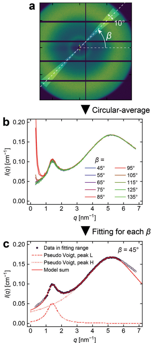
Fig. 5 Procedure for the SAXS analysis. (a) Example of the region used for sector averaging. The case of \beta = 45^\circ for B at \lambda = 1.83 is shown as an example. (b) 1D profiles at each \beta indicated, obtained by sector averaging the image in Panel a. (c) Representative example of the curve fitting for 1D profiles. The symbols are the data at \beta = 45^\circ in Panel b. The data points used for the fitting are indicated by closed symbols. Dotted, dashed, and solid curves represent two pseudo Voigt functions and their sum used for fitting, respectively.
