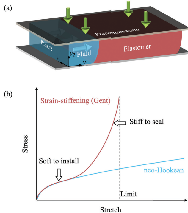
Fig. 1 Elastomeric seals. (a) An elastomer is precompressed between two rigid walls and is subject to fluid pressure. (b) Stress–stretch curves of a neo-Hookean material and a strain-stiffening material.
