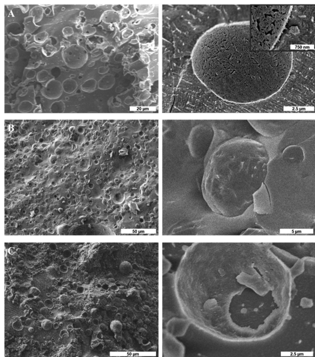
Fig. 6 Cryo SEM images of composite BSA-Ludox Cl microcapsules loaded with different oils: toluene (A), mint oil (B) and Miglyol (C).
