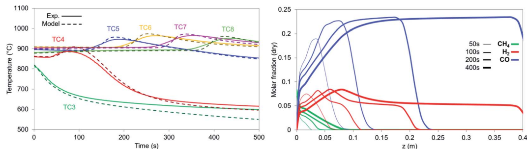
Fig. 14 (Left) Temperature profiles for the experiment (solid lines) and model (dashed lines) for reduction with synthetic biogas ( \text{CO}_2 : \text{CH}_4 - 6 : 1 ) for 900^\circ\text{C} and 1 bar. (Right) Axial molar fraction profiles during reduction with synthetic biogas \text{CO}_2 : \text{CH}_4 - 6 : 1 for 900^\circ\text{C} and 1 bar.
