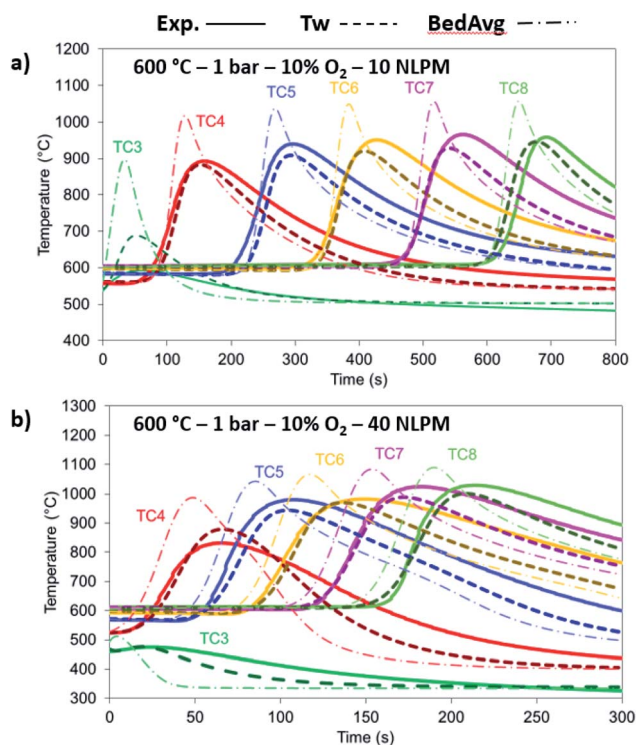
Fig. 10 Temperature comparison between the experimental (solid lines), 1-D thermowell model (dashed lines) and 1-D bed model (dashed dotted lines) temperature for 10% O 2 , 1 bar and 600 \text{ }^\circ\text{C} with (a) 10 NLPM and (b) 40 NLPM.
